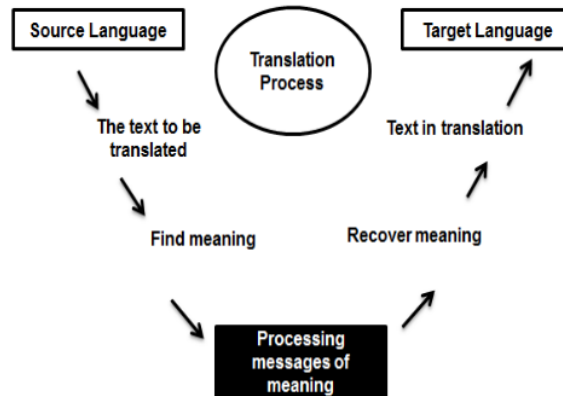
Diagram 2. Translation Process
